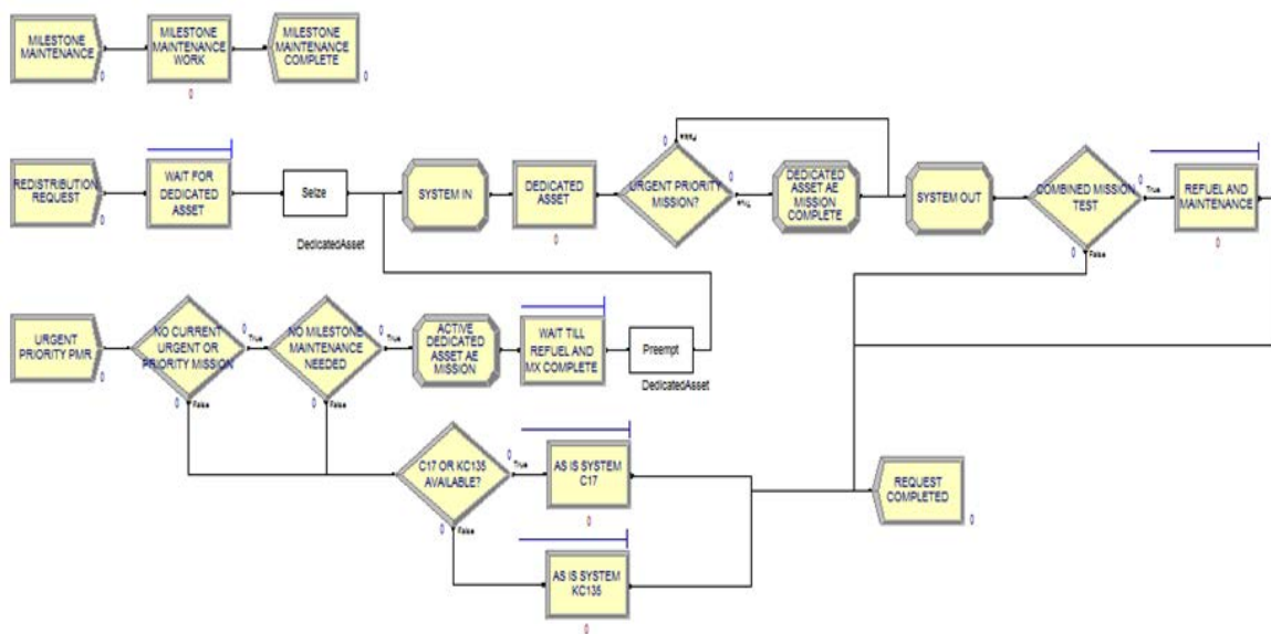
Figure 13: Simulation Model
